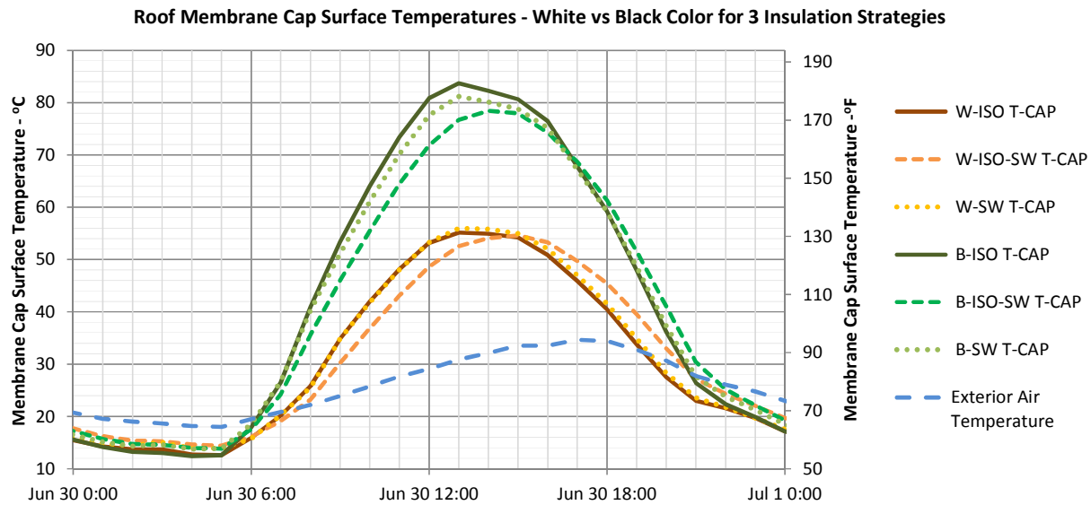
Figure 16 Roof Membrane Cap Surface Temperatures for White and Black Cap Sheet for 3 Insulation Strategies – June 30, 2013
