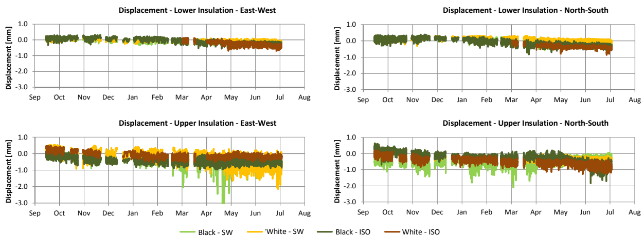
Figure 18 Insulation Displacement for Stone Wool and Polyiso Roofs (Black and White Membrane) at Lower layer and Upper Layer of Insulation in East-West and North-South Orientation.
