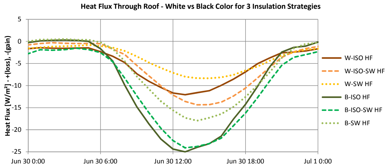
Figure 14 Comparison of Heat Flux between White and Black Cap Sheet for 3 Insulation Strategies
