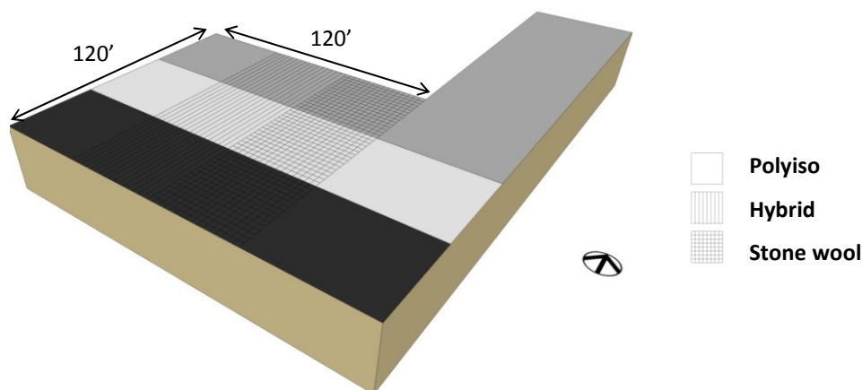
Figure 1 Study Building and Layout of Roof Membrane Cap Sheet Color and Insulation Strategy
