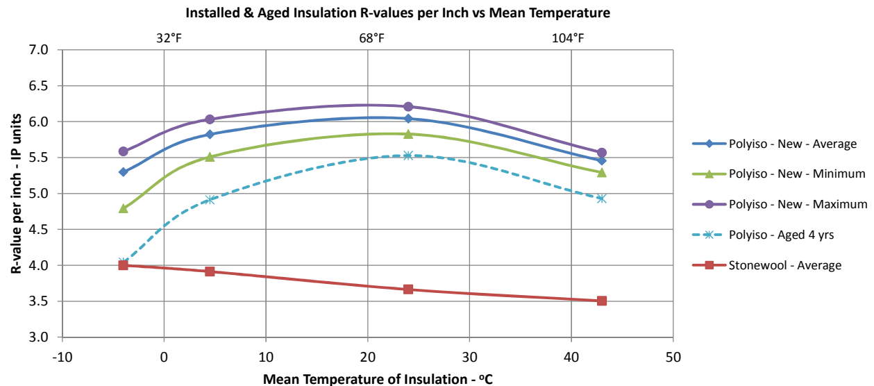
Figure 12 Apparent R-value per inch vs Mean Temperature for Polyiso and Stone Wool Insulation
