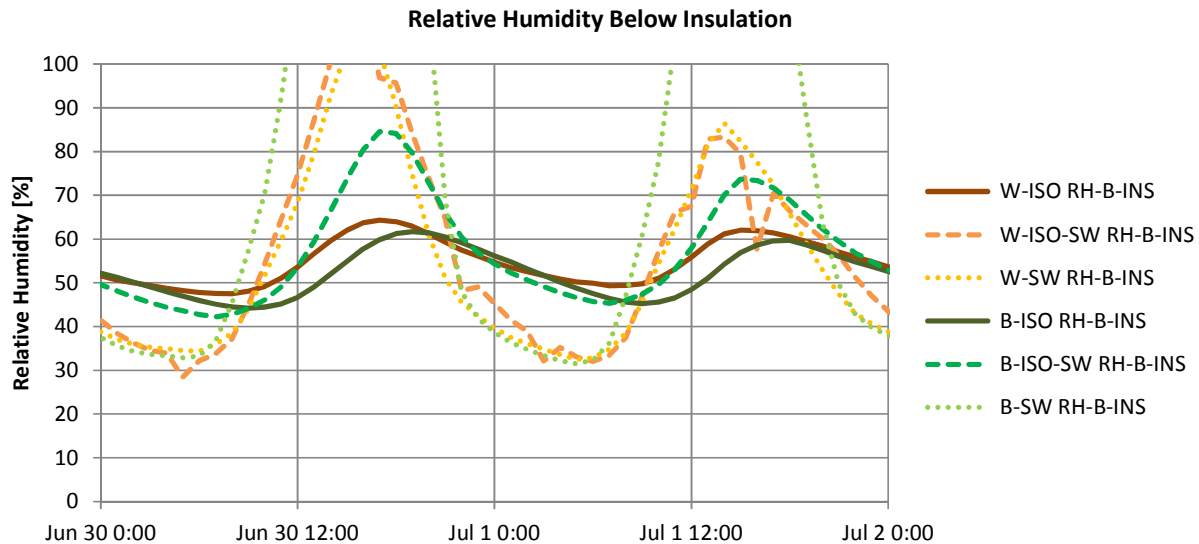
Figure 20 Hourly RH Levels below Insulation Demonstrating the Diurnal Influence of Solar Radiation on Stone Wool, Hybrid, and Polyiso Insulated Assemblies (White vs Black Membrane), June 30 and July 1, 2013.
