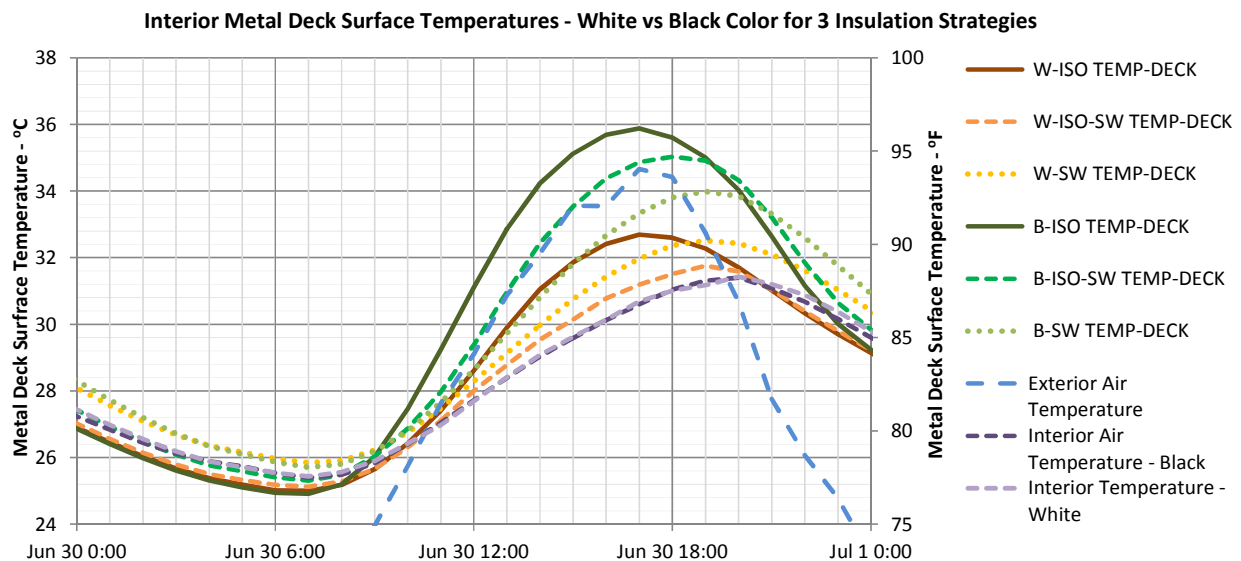
Figure 17 Interior Metal Deck Surface Temperatures for White and Black Cap Sheet for 3 Insulation Strategies – June 30, 2013
