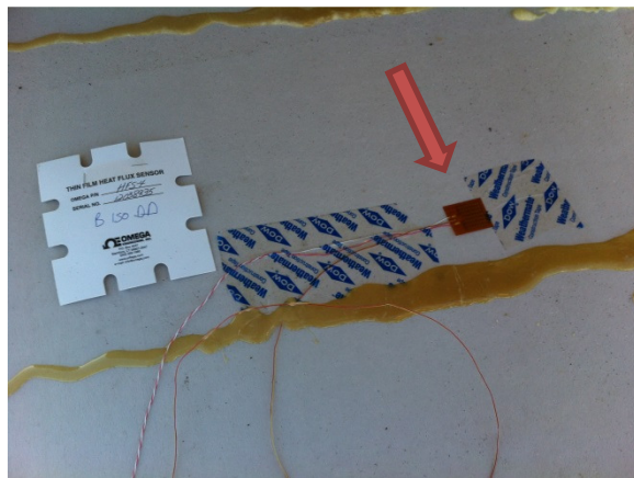
Figure 9 Heat flux sensor between layers of insulation.
