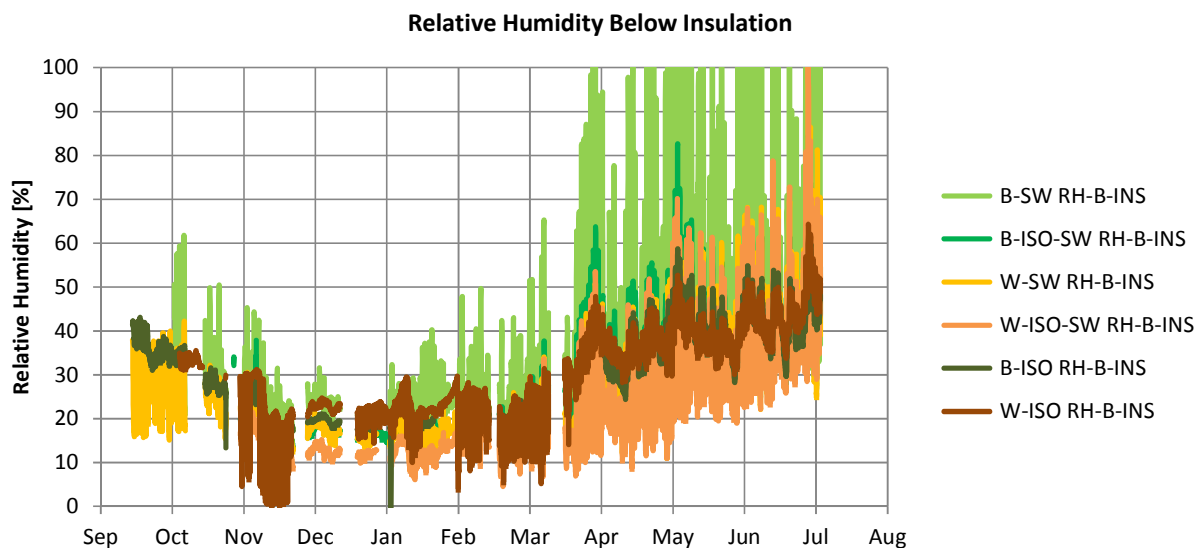
Figure 19 Relative Humidity Below Insulation, Sorted from Highest to Lowest RH Levels – September 15, 2012 through July 3, 2013
