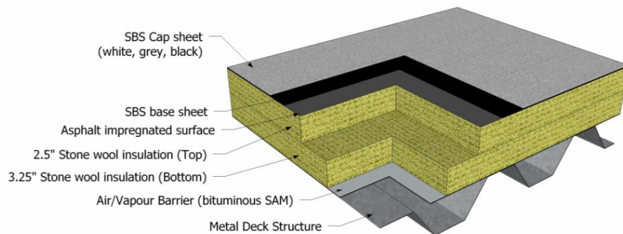
Figure 3 Stone Wool Roof Assembly (5.75" stone wool, R-21.4) – Weight: 26.7 kg/m 2 , Heat Capacity: 22.7 kJ/K/m 2
