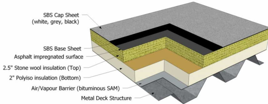
Figure 4 Hybrid Roof Assembly (2.5" stone wool over 2" polyiso, R-21.3) – Weight: 14.3 kg/m 2 , Heat Capacity: 13.7 kJ/K/m 2
