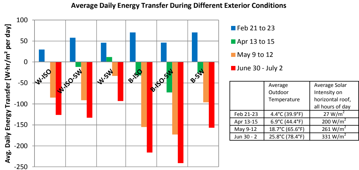
Figure 15 Average Daily Energy Transfer for Selected Dates through White and Black Cap Sheet for 3 Insulation Strategies
