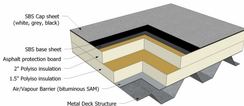
Figure 2 Polyiso Roof Assembly (3.5" polyiso, R-21.5) – Weight: 4.6 kg/m 2 , Heat Capacity: 6.75 kJ/K/m 2
