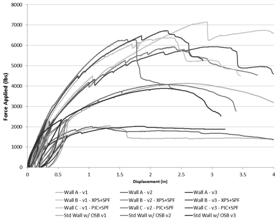
FIGURE 1: STRUCTURAL TESTING COMPARISON SUMMARY GRAPH
